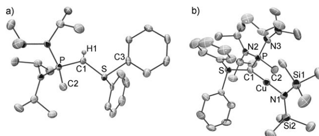
Figure 1. X-ray crystal structures of 2 (a) and 5 (b). H atoms and the triflate anion (for 2 ) are omitted for clarity. [8] Thermal ellipsoids are drawn at the 50% level. Selected bond lengths [Å] and angles [°]. 2 : P–C1 1.721(5), S–C1 1.690(4), P–C2 1.796(4), S–C3 1.810(5), P–C1–S 118.0(3). 5 : P–C1 1.709(5), S–C1 1.677(5), P–C2 1.804(5), C1–Cu 1.903(4), N1–Cu1 1.874(4), P–C1–S 115.3(2), C1–Cu–N 176.97(18), S–C1–Cu 125.7(3), P–C1–Cu 118.7(2).
