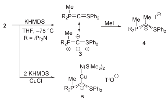
Scheme 2. Synthesis and reactivity of bisylide 3 .
