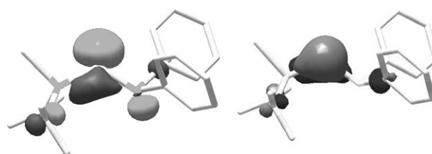
Figure 3. Highest occupied molecular orbitals of 6 : HOMO (left) and HOMO-1 (right).
