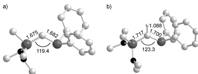
Figure 2. Structures of 6 (a) and 7 (b) optimized at the B3LYP/6-31+G(d,p) level of calculation. Interatomic distances are in Å and bond angle in degrees. H atoms and the triflate anion (for 7 ) are omitted for clarity.
